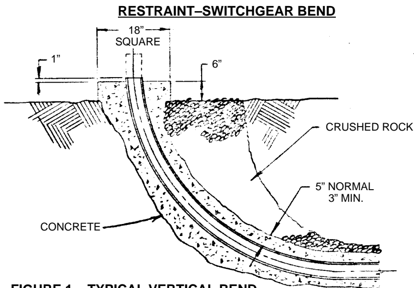
FIGURE 1 – TYPICAL VERTICAL BEND SIDE ELEVATION
