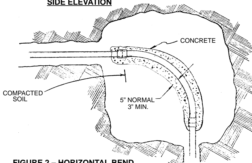
FIGURE 2 – HORIZONTAL BEND PLAN VIEW
